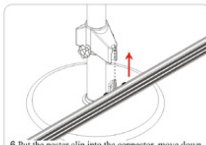
6. Put the poster clip into the connector, move down the connector and make the screw tight to fasten the clip
